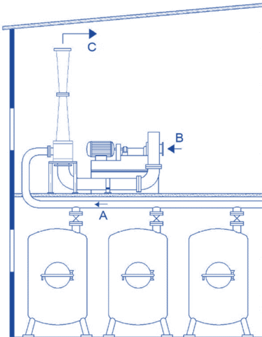
A = exhaust B = air C = to exhaust gas cleaning plant
